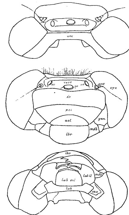
FIG. 2.— Podogomphus praetorius . Dorsal, frontal and ventral views of head. Lettering as in Text-fig. 1.
